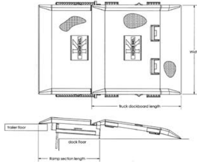
2-PIECE STEEL DOCKBOARD
