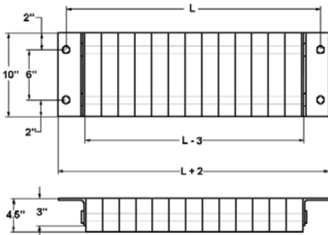
4" PROJECTION HORIZONTAL MOUNT
