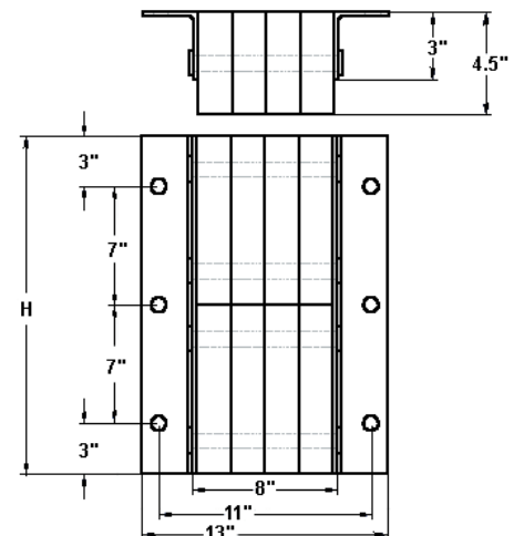
4" PROJECTION VERTICAL MOUNT
